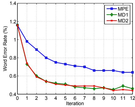
Fig. 1. Performance comparison on TIDIGITS test set
