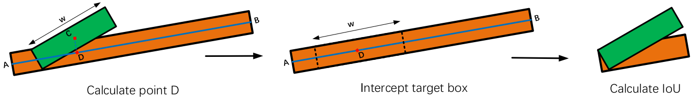
Fig. 5. Details of LIIoU calculation, green bounding box is proposed bounding box, orange bounding box is target box.
