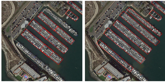
Fig. 7. Comparison of LIIoU and IoU. (From left to right) Calculate overlaps with IoU in the first R-CNN, calculate overlaps with LIIoU in the first R-CNN (overlaps are both calculated with IoU in the last R-CNN).
